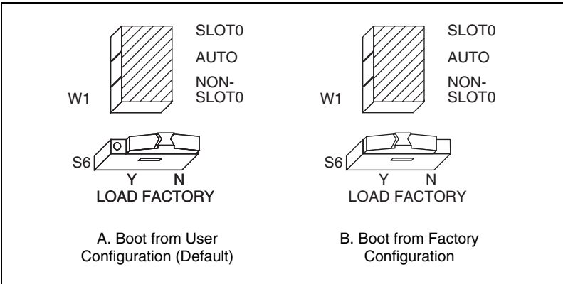
Figure C-3. EEPROM Operation
