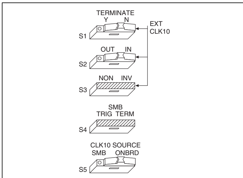
Figure C-4. Generate Internal CLK10 and Drive to the Backplane
